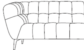
2 Seater Left Arm (available as right arm) W147 x D95x H76cm
